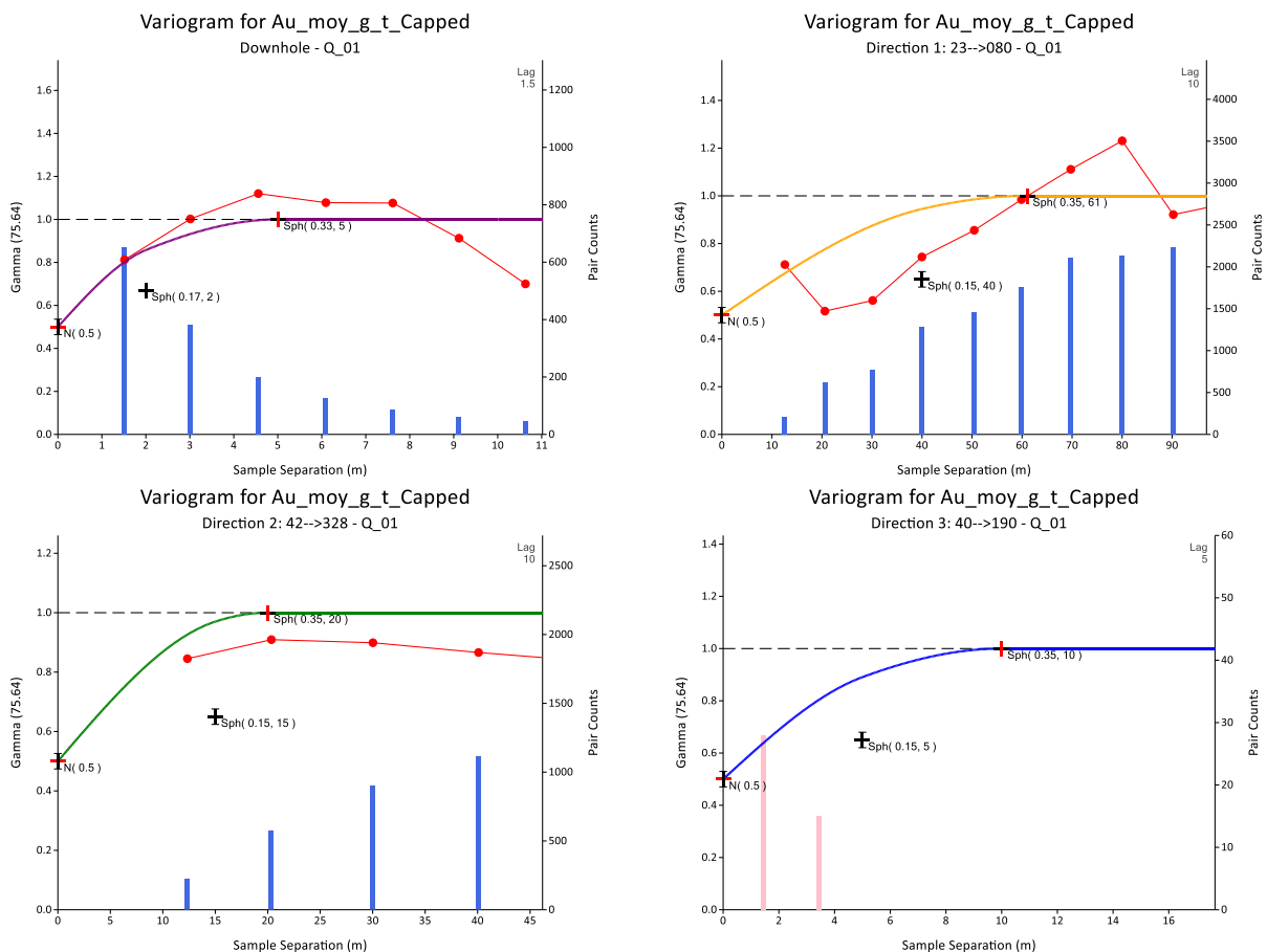
Figure 14-17: Example of the variography study for the Q_01 zone
