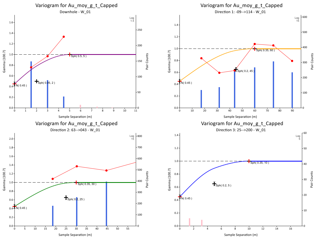
Figure 14-15: Example of the variography study for the W_01
