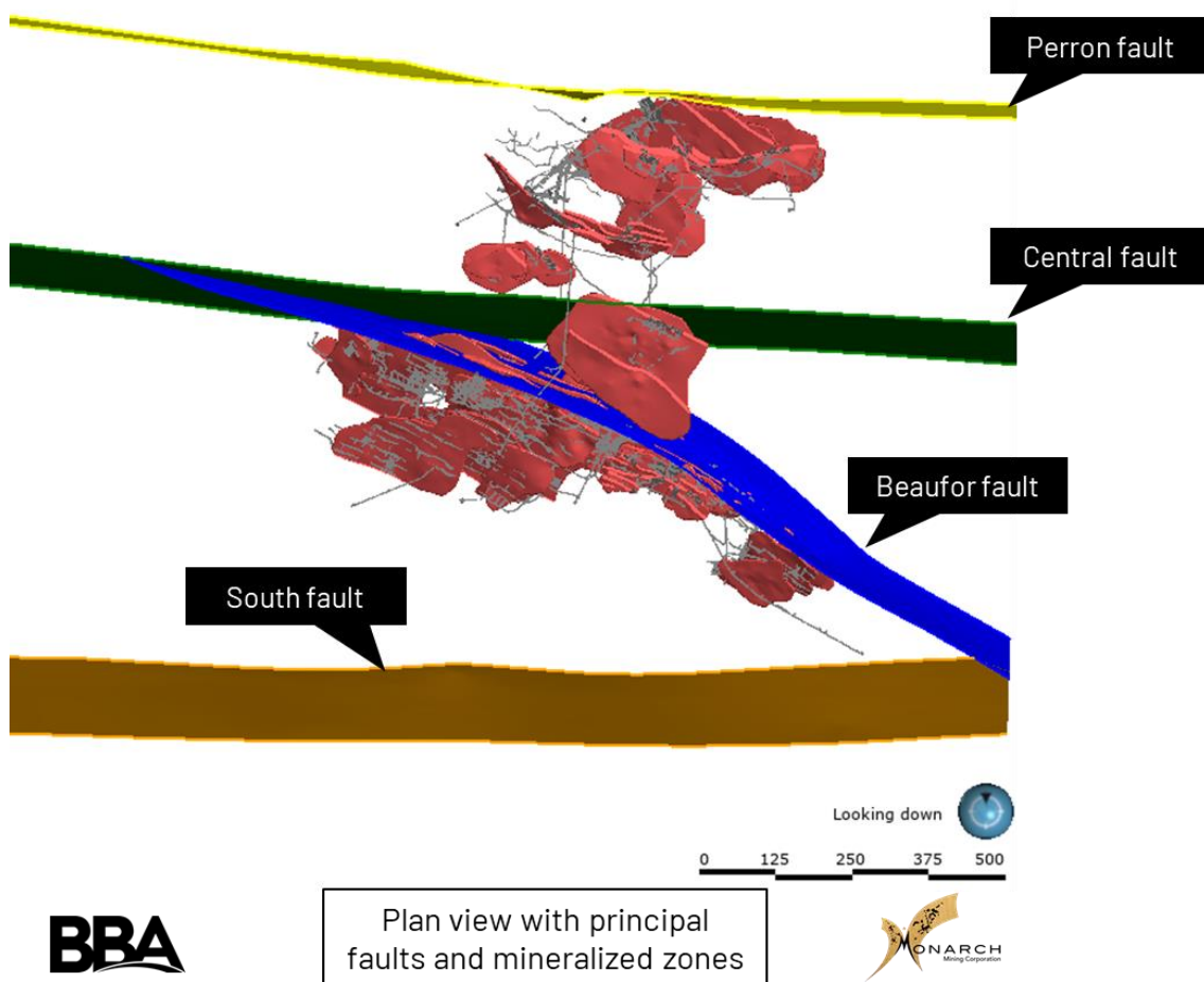
Figure 7-5: Plan view of the Beaufor Mine with the 3D modelled principal fault zones
