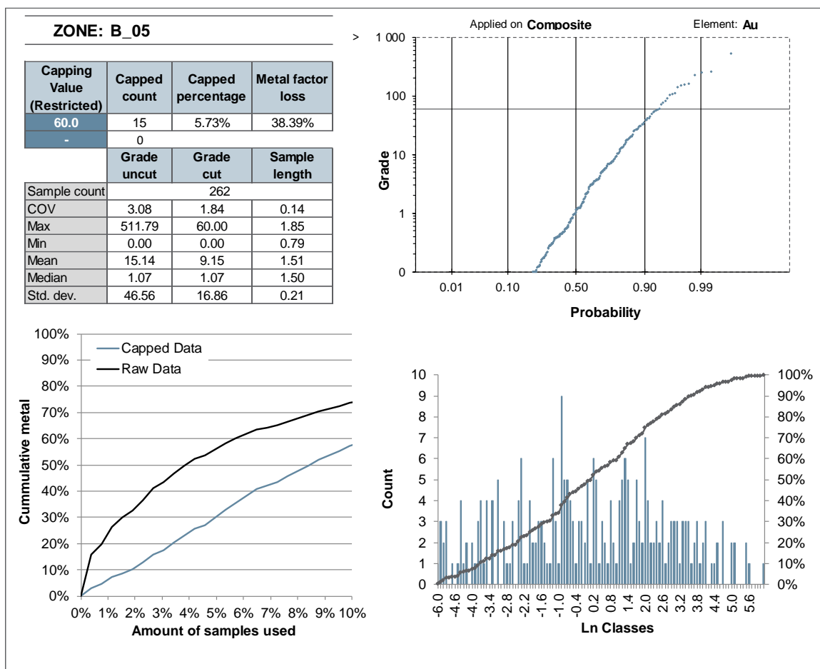
Figure 14-10: Graphs supporting capping threshold decisions on composites for the B_05 zone
