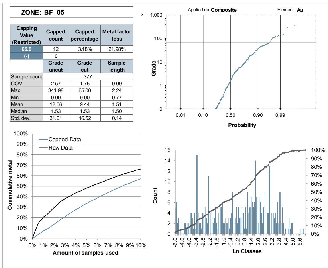
Figure 14-11: Graphs supporting capping threshold decisions on composites for the BF_05 zone
