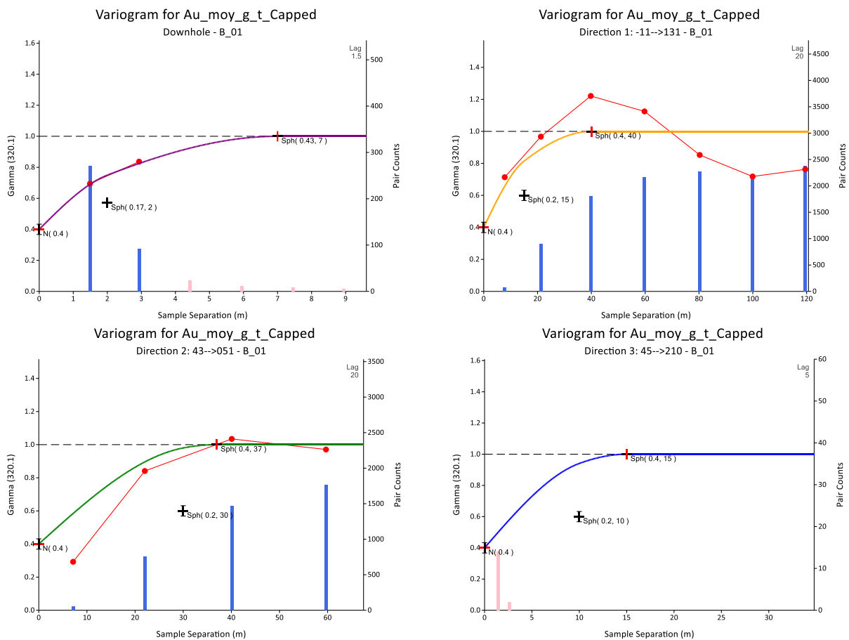
Figure 14-16: Example of the variography study for the B_01 zone
