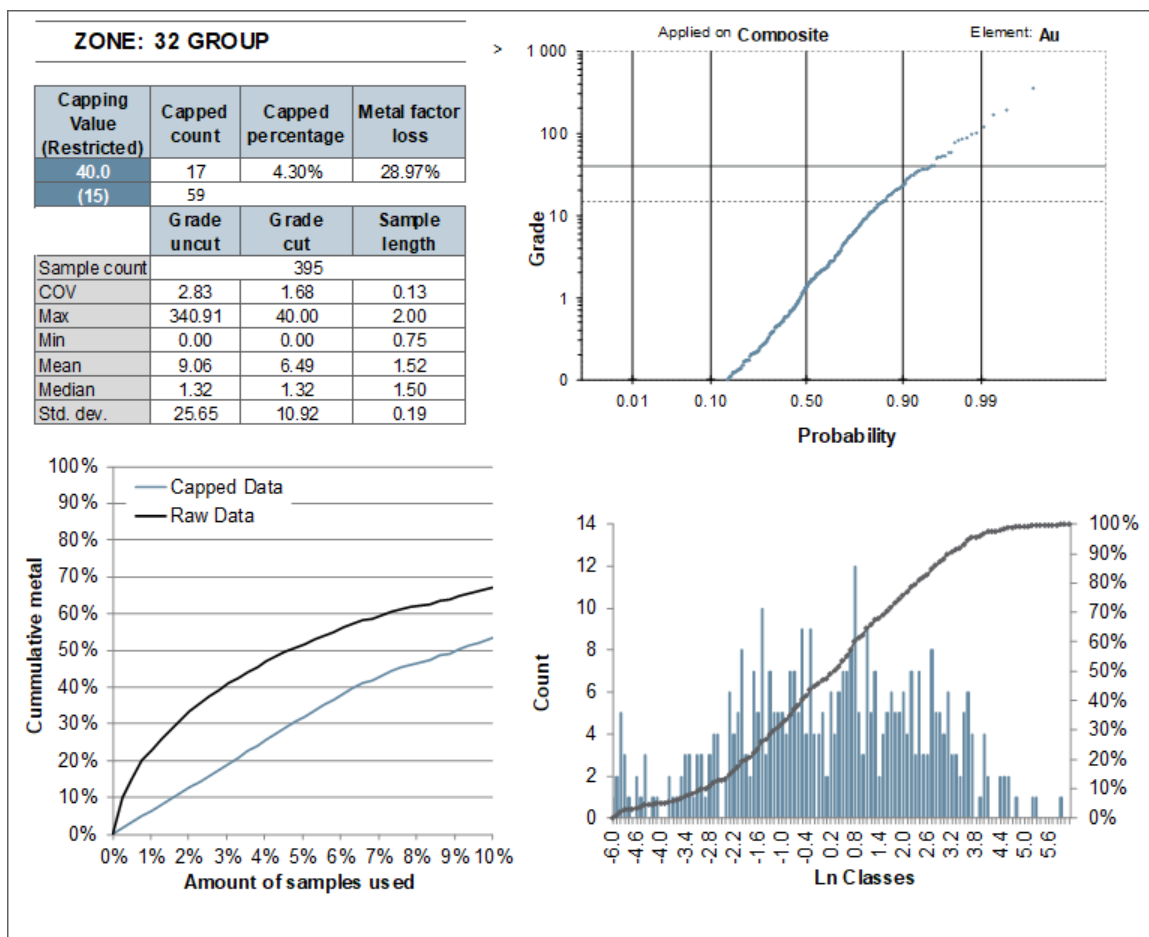
Figure 14-12: Graphs supporting capping threshold decisions on composites for the 32 group of zones
