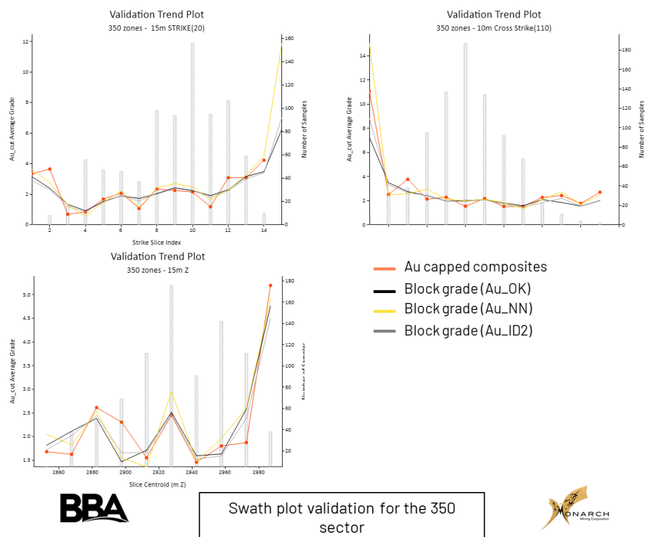
Figure 14-22: Example of block model validation swath plots for the 350 sector
