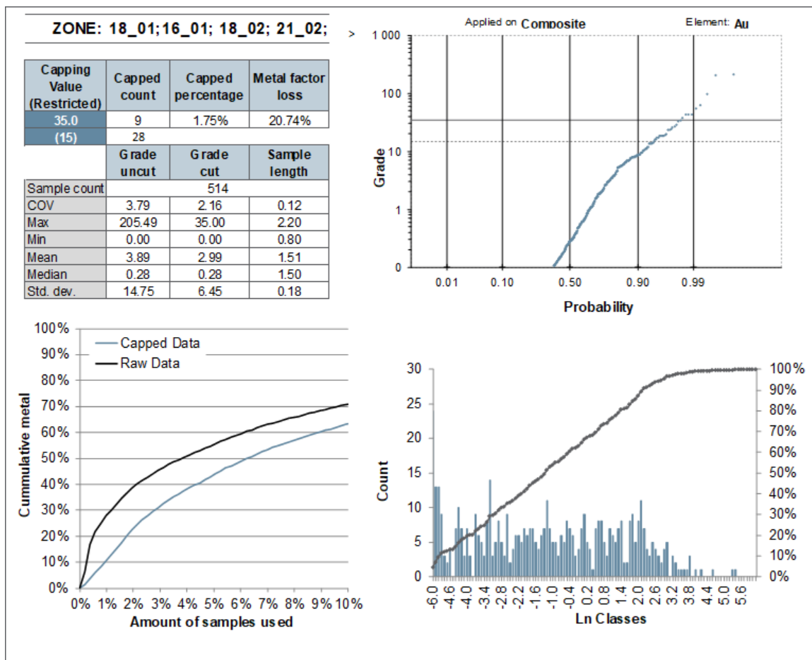
Figure 14-7: Graphs supporting capping threshold decisions on composites for the 18_01 group of zones
