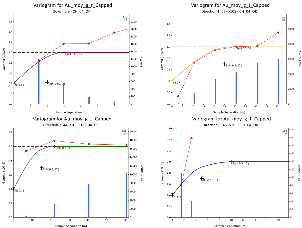
Figure 14-14: Variograms for Au for CH_04
