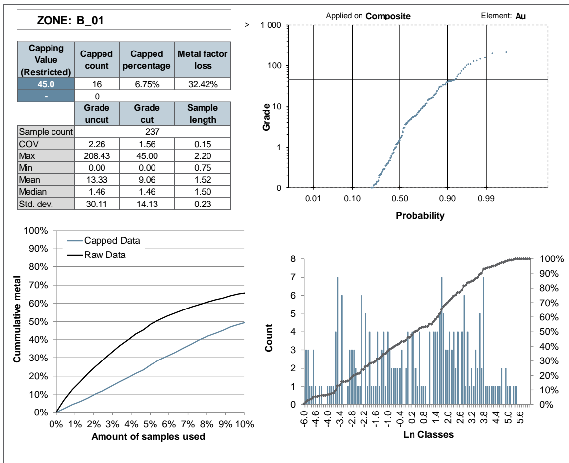
Figure 14-9: Graphs supporting capping threshold decisions on composites for the B_01 zone
