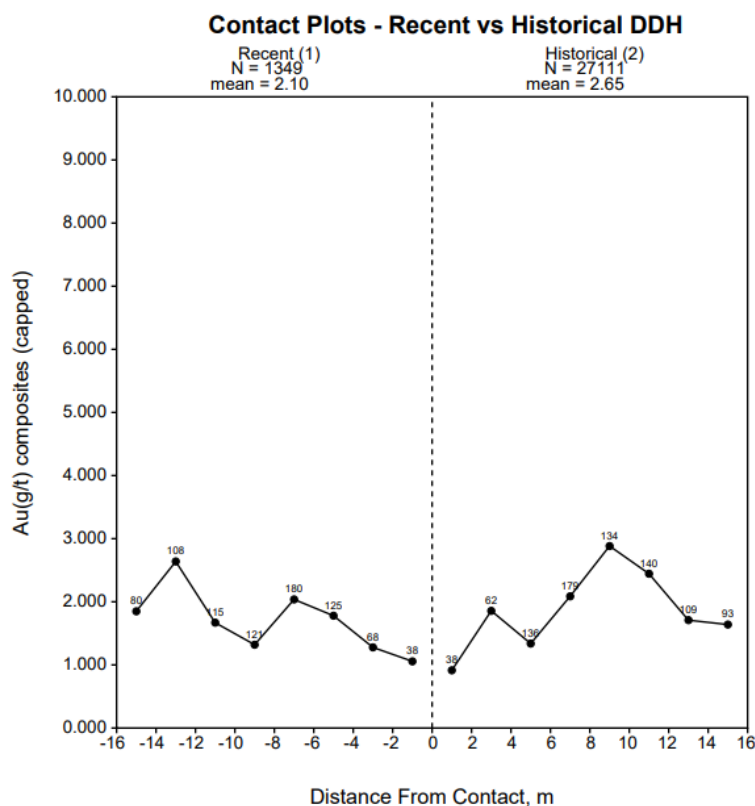
Figure 14-13: Contact analysis on the capped composites between the historical and recent diamond drillholes
