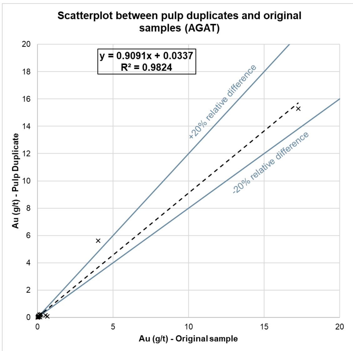
Figure 11-1: Scatterplot between pulp duplicates and original samples for the 2020-2021 drilling campaigns (n=27)
