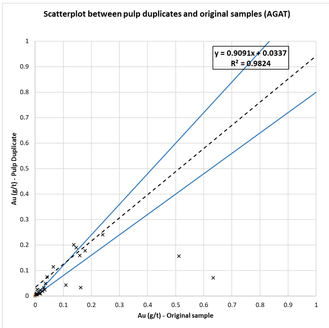
Figure 11-2: Close-up view of Figure 11-1 of the scatterplot comparing original samples to pulp duplicates for the 2020-2021 drilling campaigns (n= 27)
